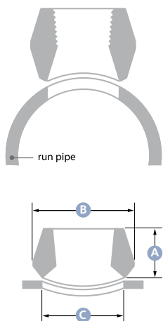
Thredolet Reducing
