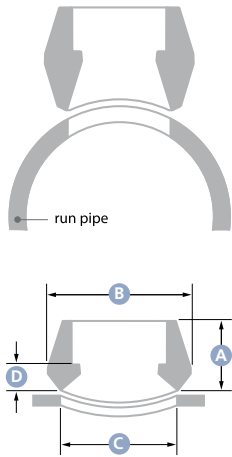
Sockolet Reducing
