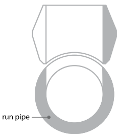
Weldolet Size on Size
